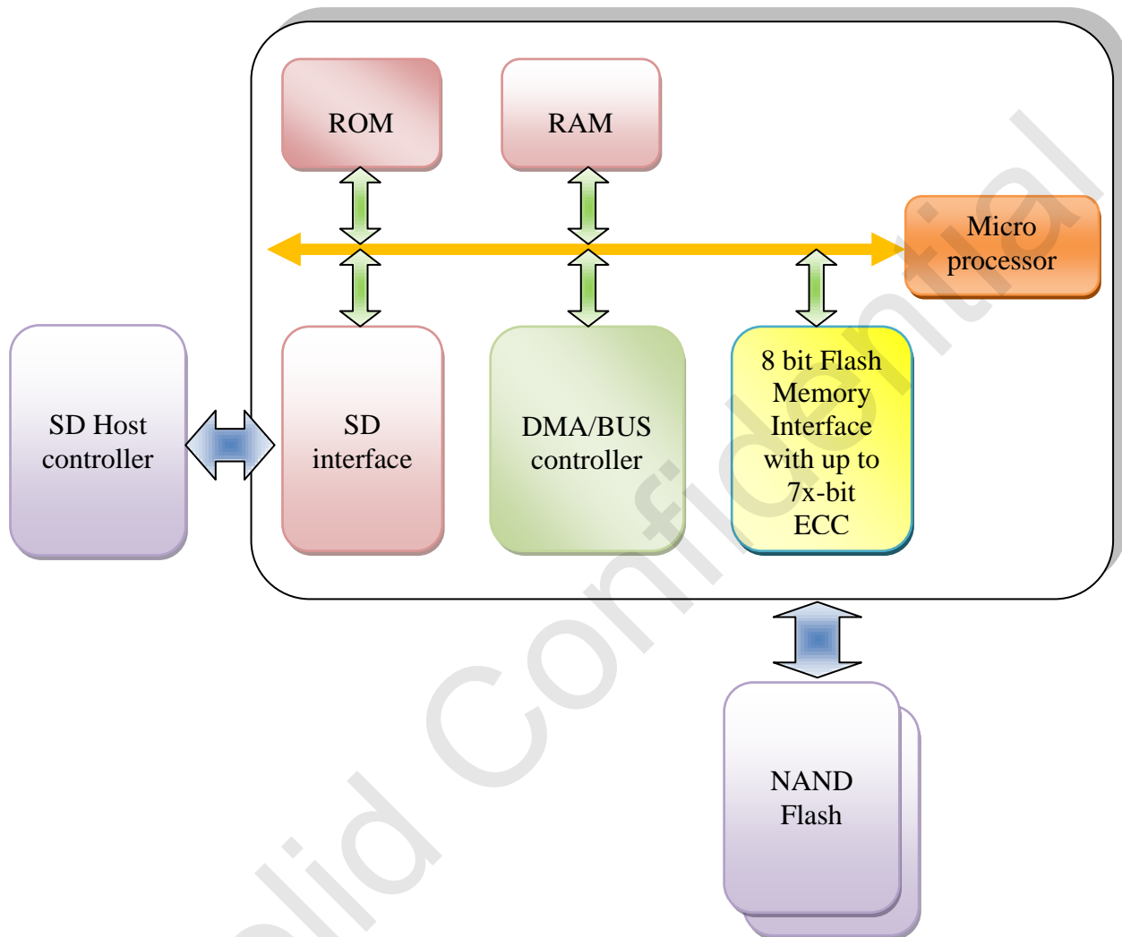
Figure 3-1 AS2703EN-DI Function Block Diagram
