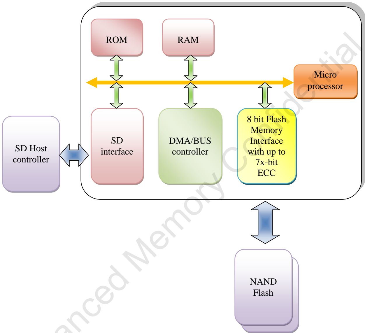
Figure 3-1 AM2703ENLT Function Block Diagram
