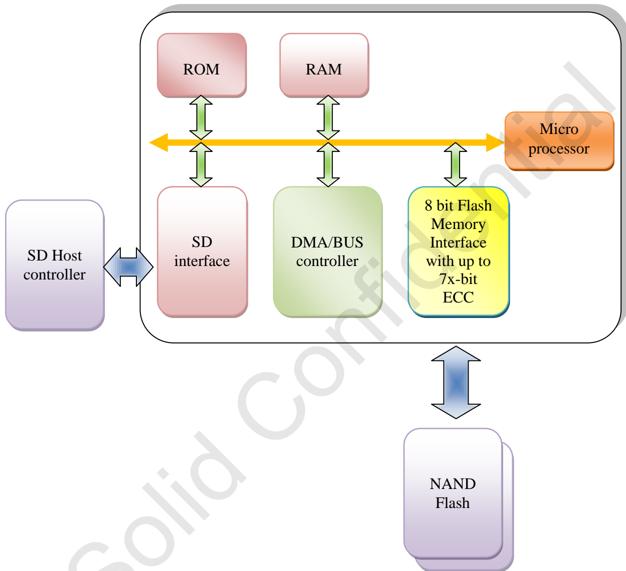
Figure 3-1 AK2689 Function Block Diagram
