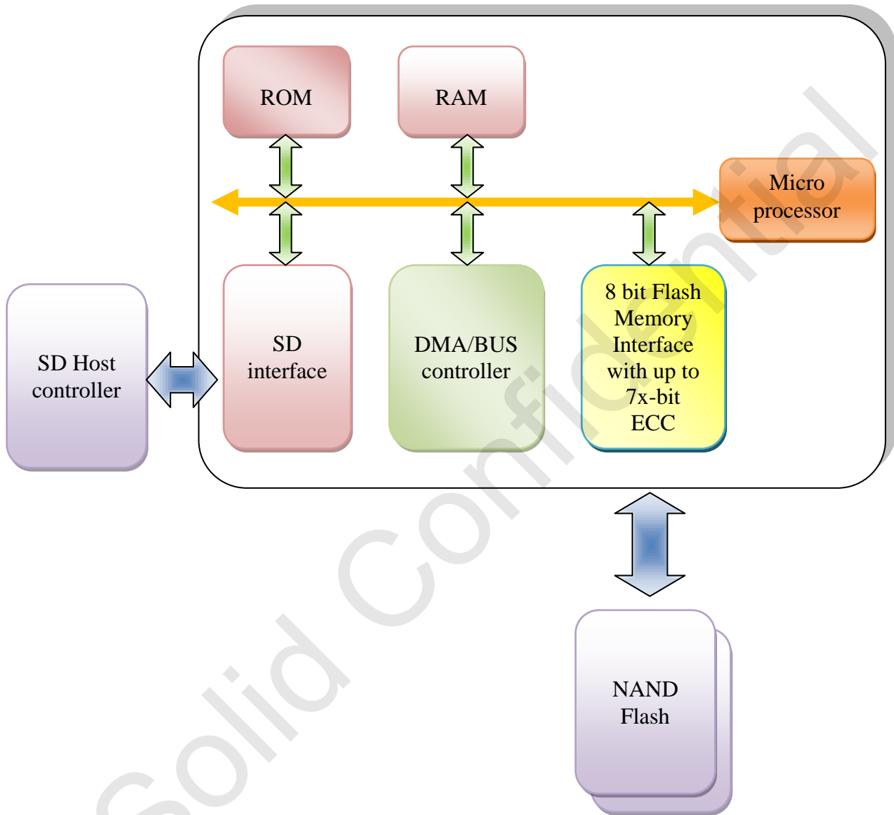
Figure 3-1 AK2703 Function Block Diagram
